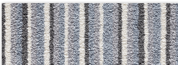
▲ 38 - Ocean Stripes
