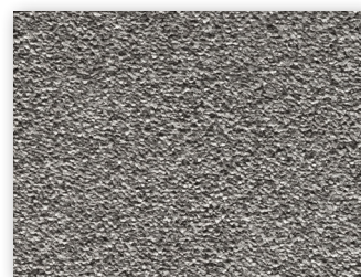
▲ 960 - Weathervane
